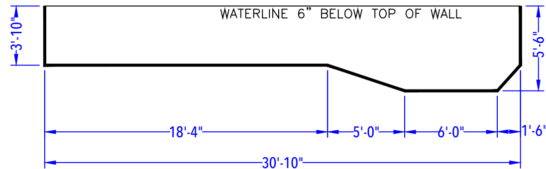
DEPTH DETAIL
