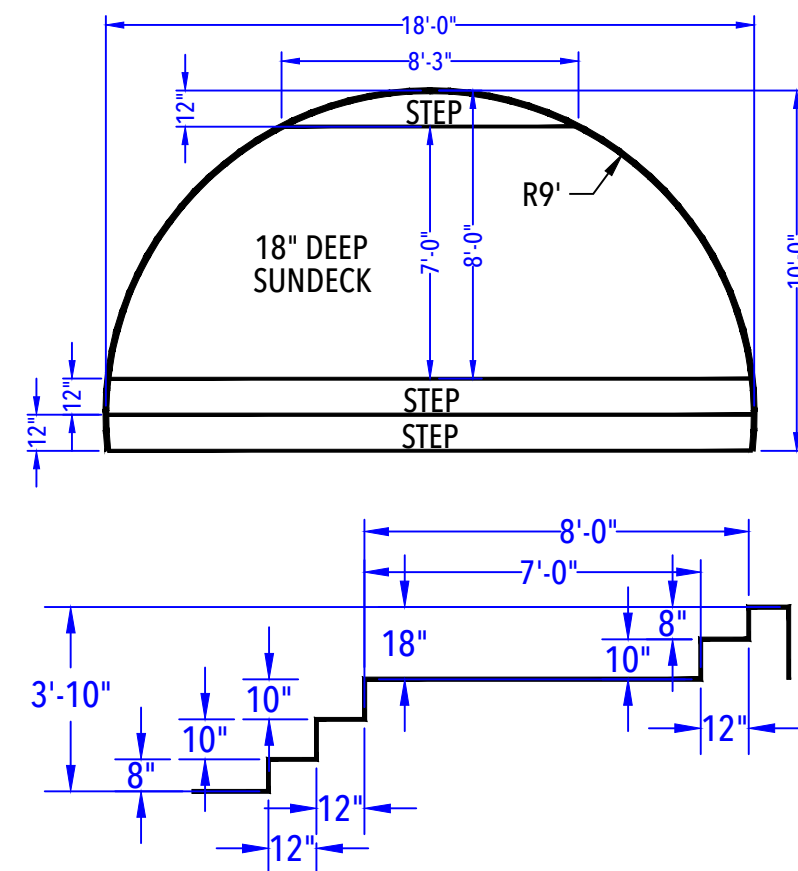
SUN DECK & ENTRY STEP DETAIL (After Concrete & Liner) N.T.S.
