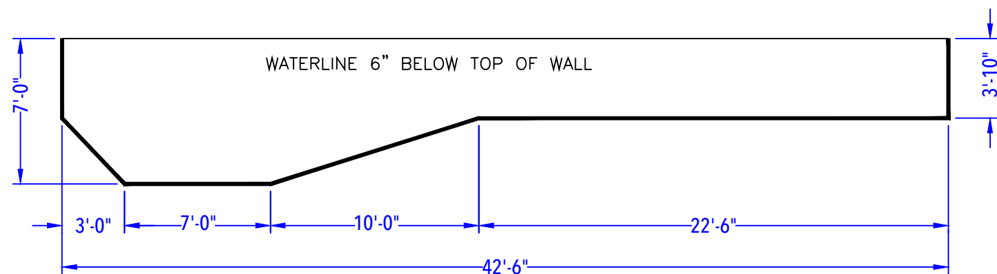
DEPTH DETAIL
