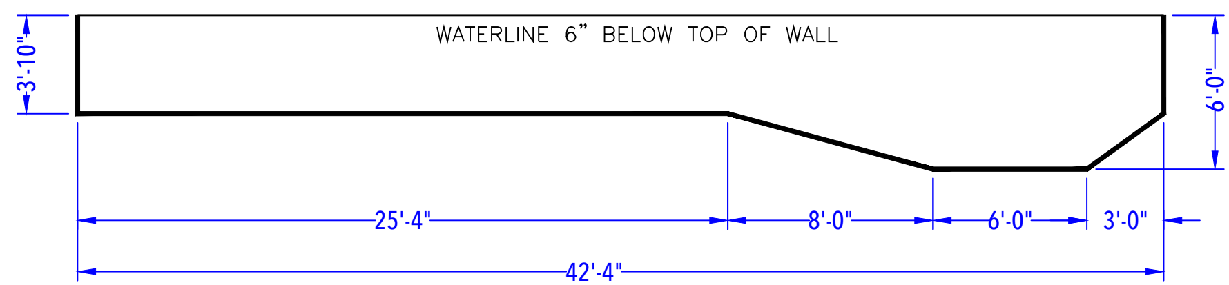
DEPTH DETAIL
