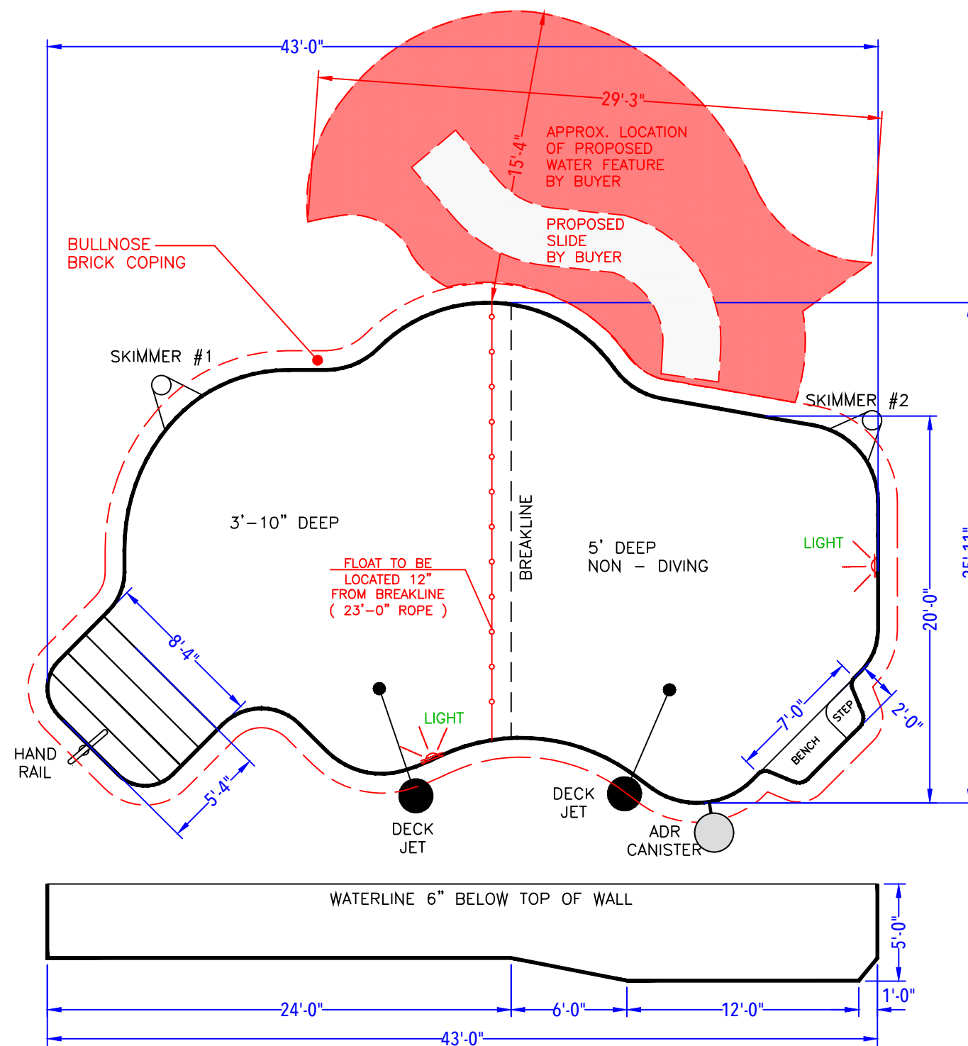
DEPTH DETAIL
