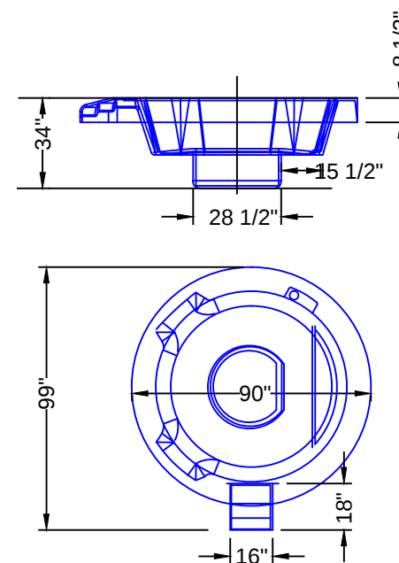
90" ROUND FIBERGLASS SPILLOVER SPA DETAIL (After Concrete & Liner) N.T.S.
