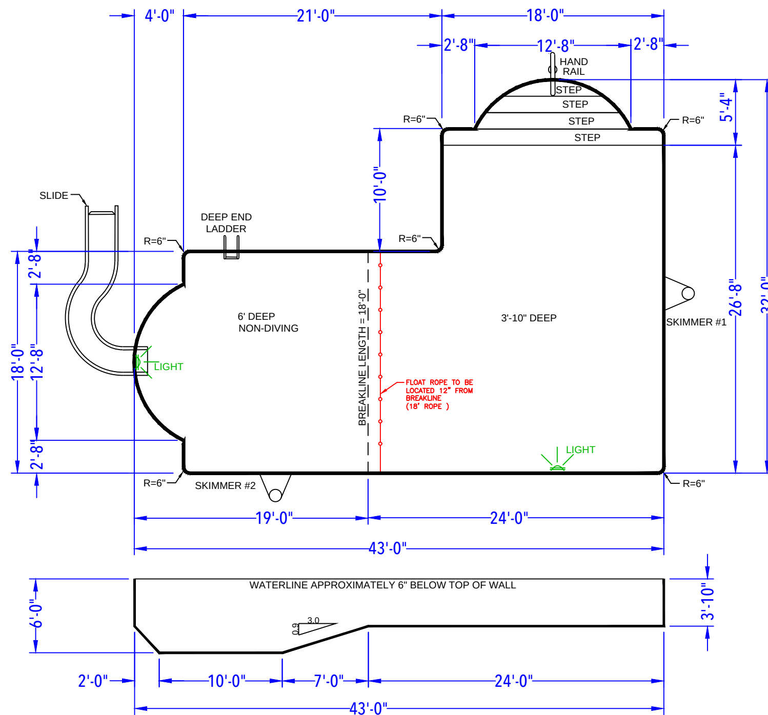
DEPTH DETAIL
