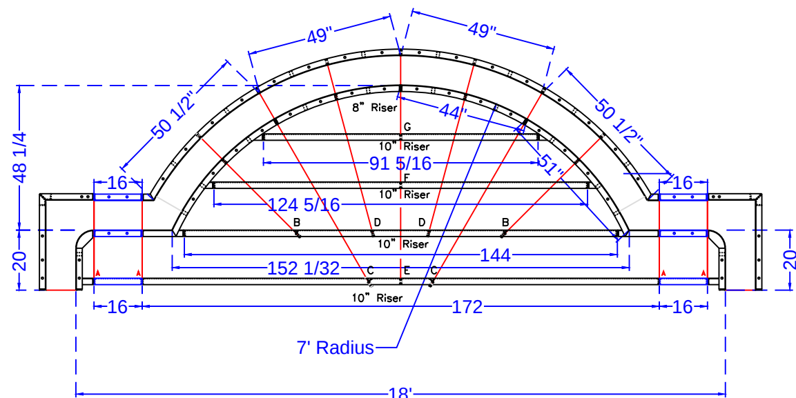
18' ROMAN END STEP ASSEMBLY SHOWN x 48
