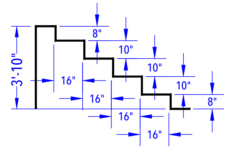
ENTRY STEP DETAIL (After Concrete & Liner) N.T.S.
