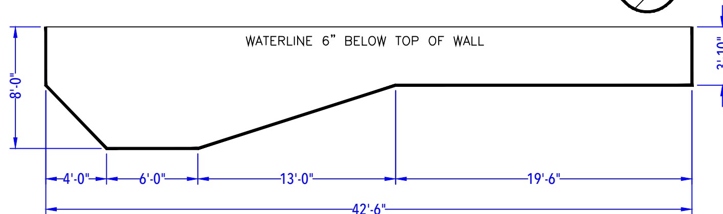
DEPTH DETAIL
