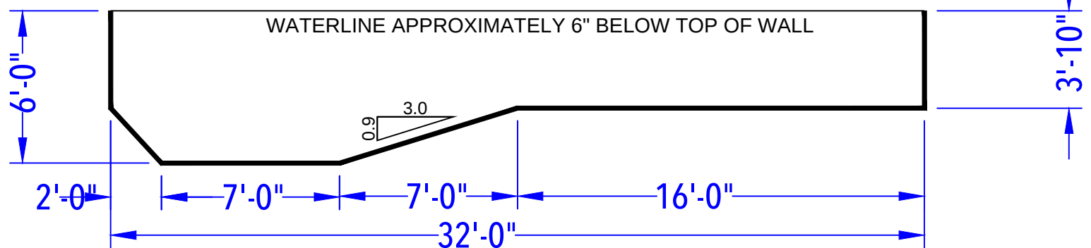
DEPTH DETAIL
