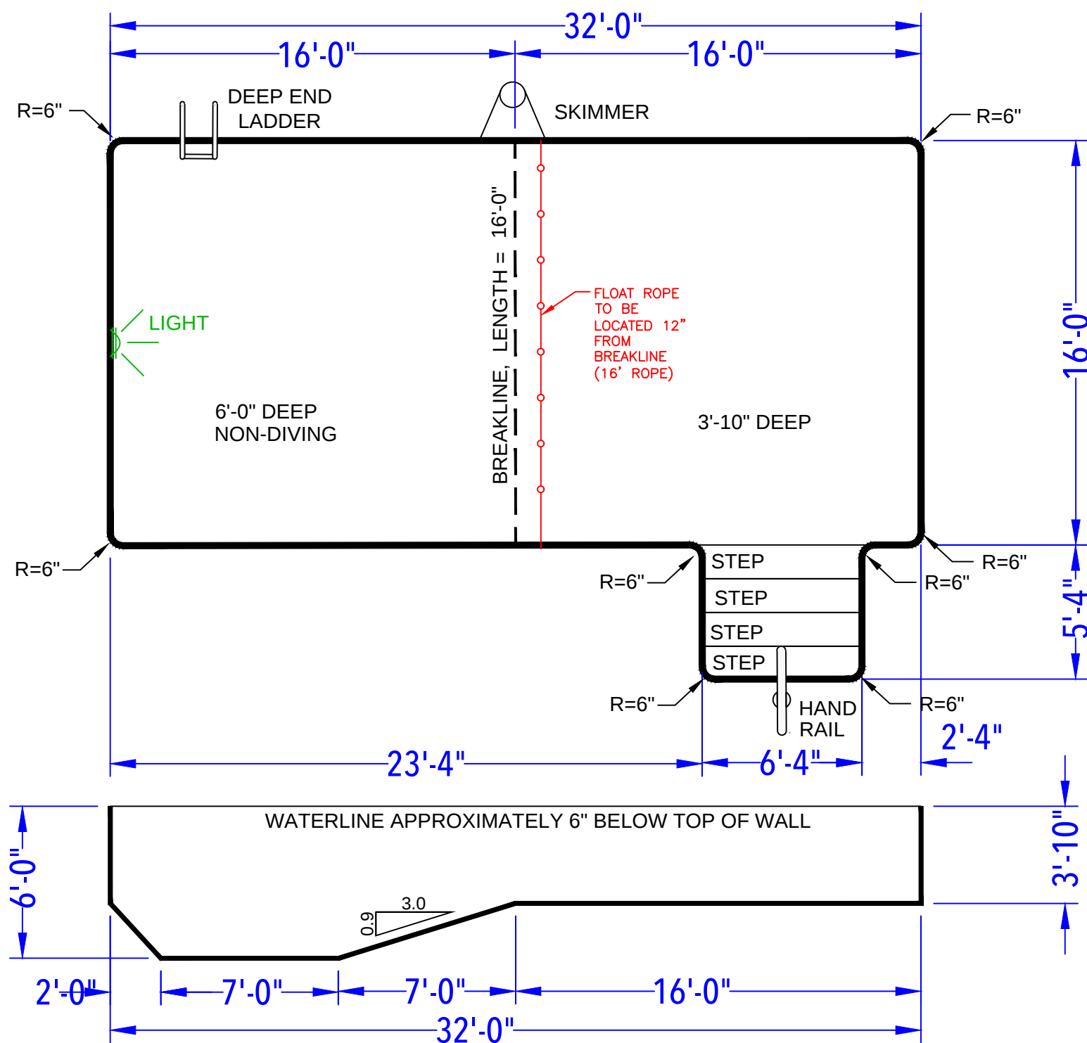
DEPTH DETAIL
