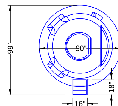
90" ROUND FIBERGLASS SPOILOVER SPA DETAIL (After Concrete & Liner) N.T.S.
