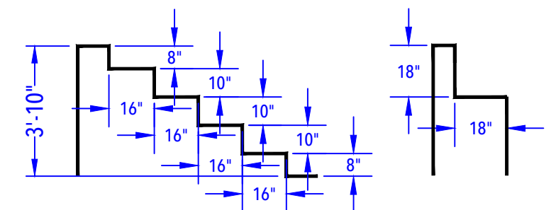
CORNER ENTRY STEP & BENCH DETAIL (After Concrete & Liner) N.T.S.
