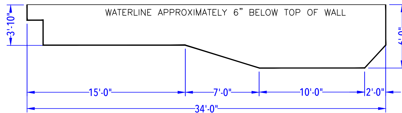
DEPTH DETAIL
