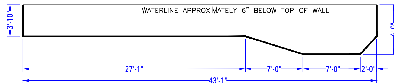
DEPTH DETAIL
