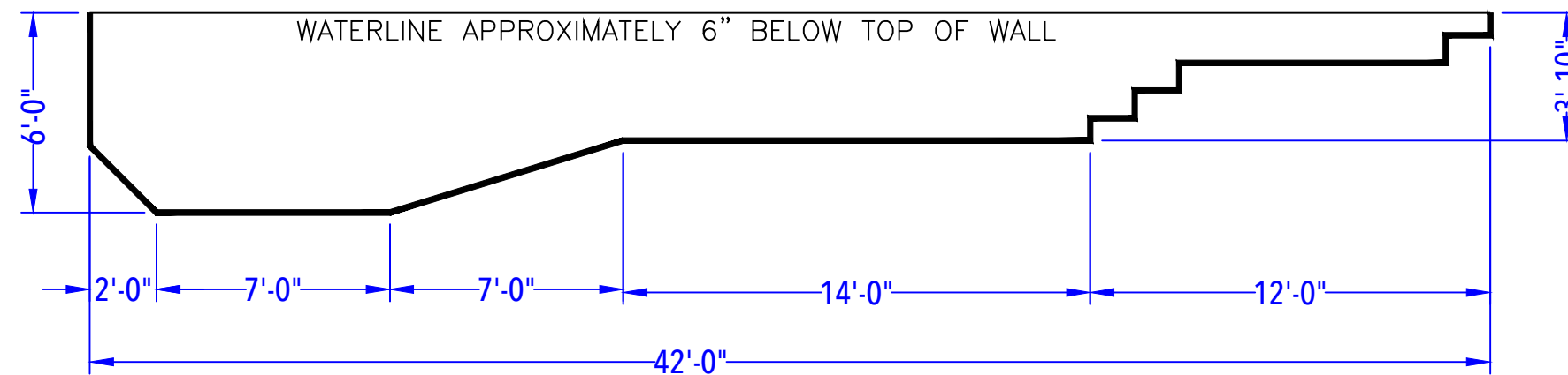
DEPTH DETAIL
