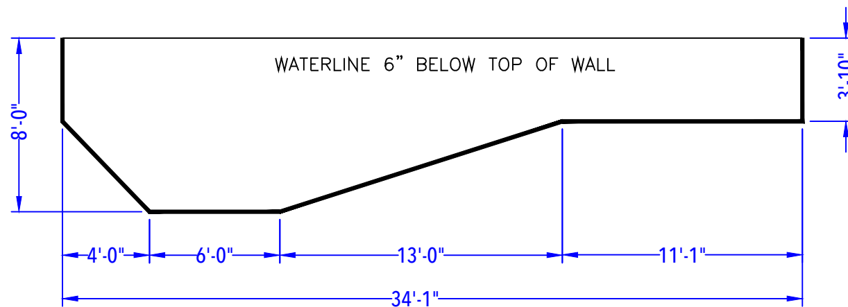
DEPTH DETAIL
