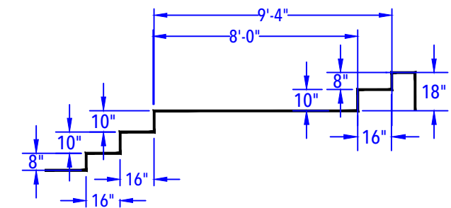
ENTRY STEP DETAIL (After Concrete & Liner) N.T.S.
