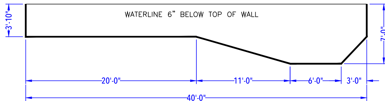
DEPTH DETAIL
