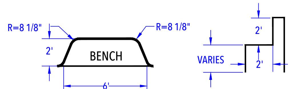
DEEP END BENCH DETAIL
