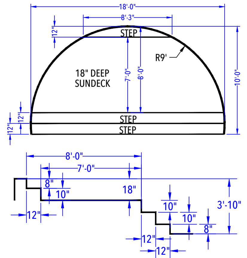
SUN DECK & ENTRY STEP DETAIL
