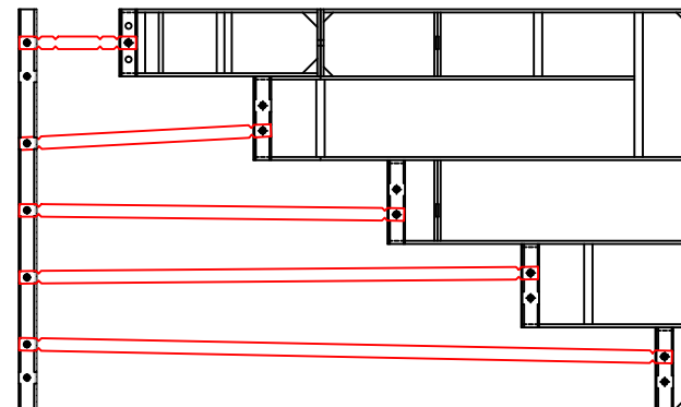
8'-4" x 5'-4" Outside End Step - 6" Radius Corners
