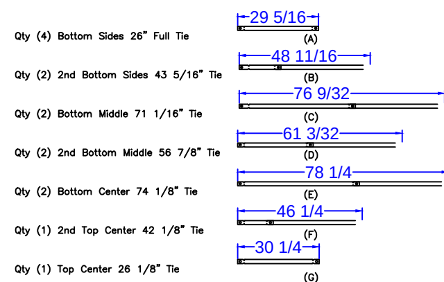
18' ROMAN END STEP - TIES SCALE: 1' = 1/4"
