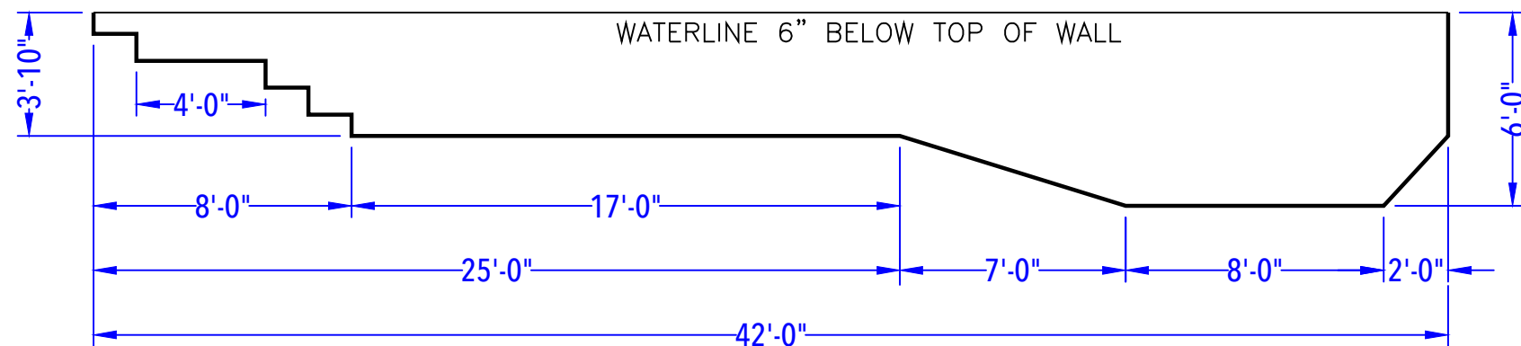
DEPTH DETAIL
