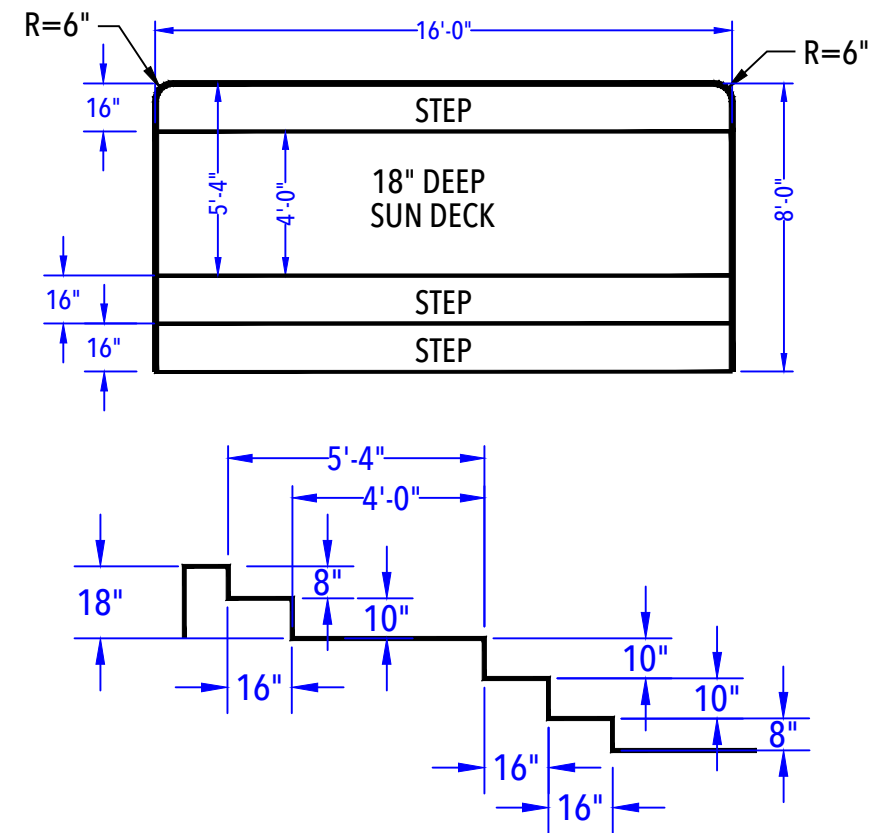
SUN DECK & ENTRY STEP DETAIL (After Concrete & Liner) N.T.S.
