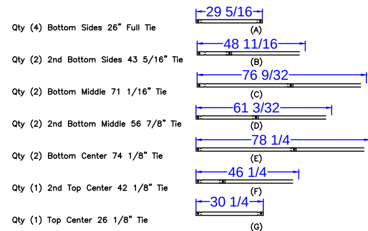
18' ROMAN END STEP - TIES SCALE: 1' = 1/4"
