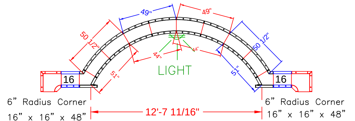
18' ROMAN END ASSEMBLY SHOWN x 48 SCALE: 1' = 1/4"
