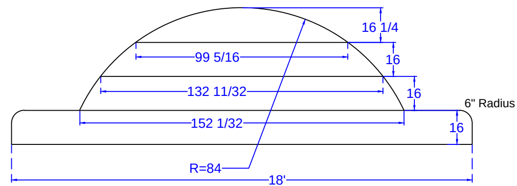
STEP DETAIL SCALE: 1' = 1/4"
