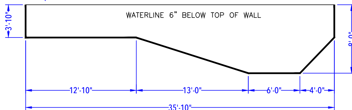
DEPTH DETAIL
