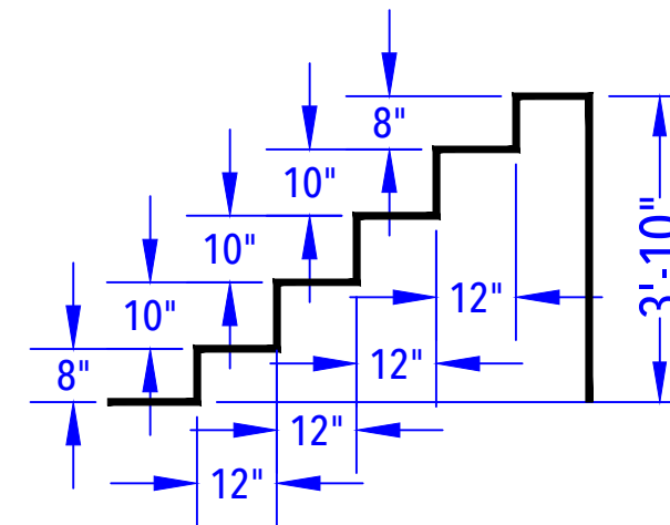
ENTRY STEP DETAIL (After Concrete & Liner) N.T.S.
