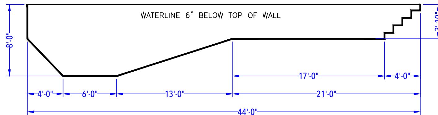
DEPTH DETAIL
