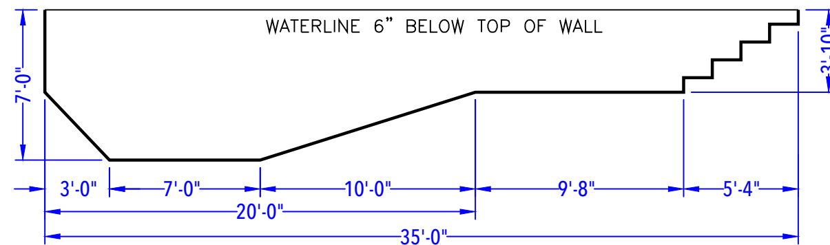
DEPTH DETAIL
