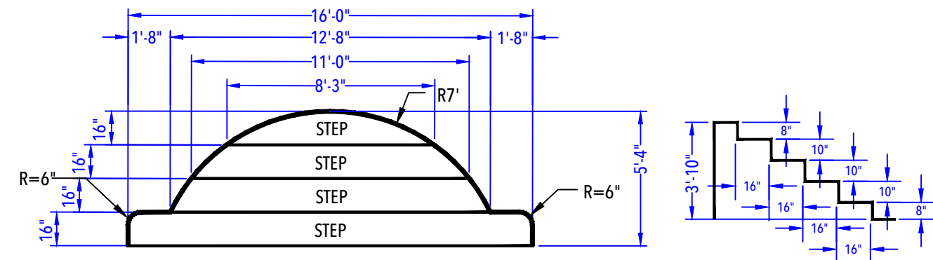
ENTRY STEP DETAIL (After Concrete & Liner) N.T.S.
