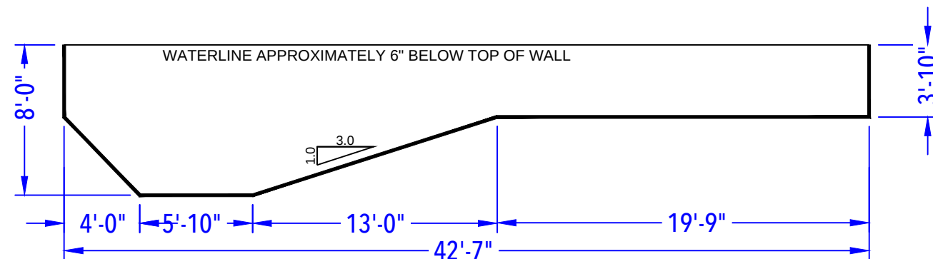
DEPTH DETAIL
