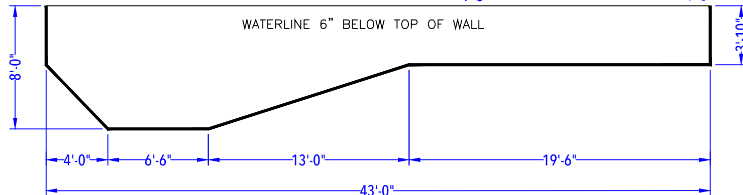
DEPTH DETAIL
