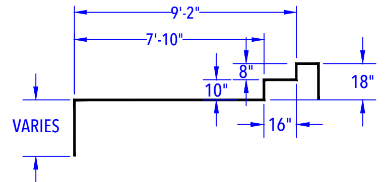
SUNDECK DETAIL (After Concrete & Liner) N.T.S.
