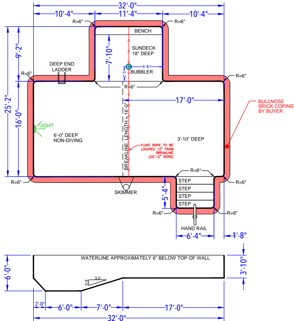
DEPTH DETAIL
