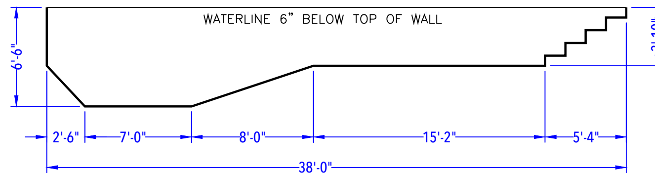
DEPTH DETAIL
