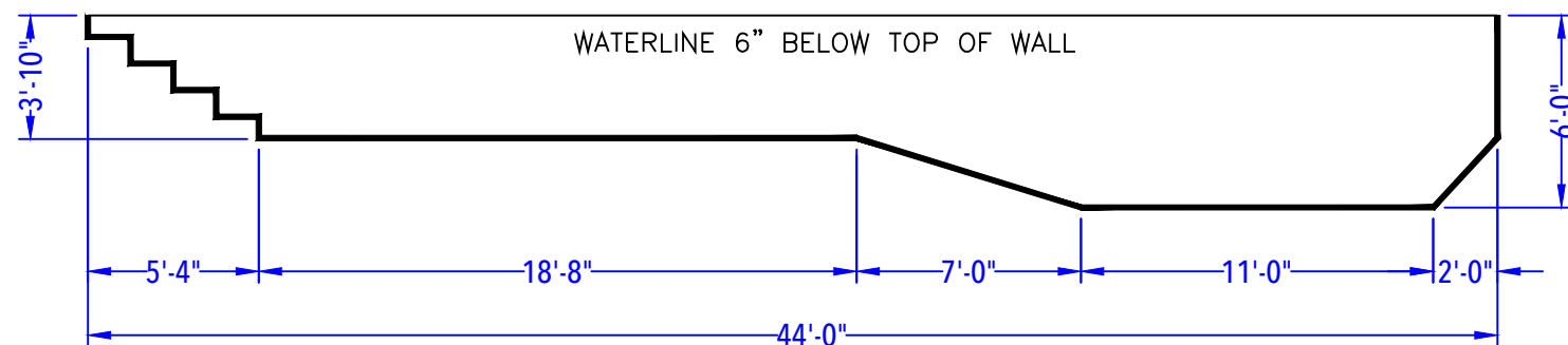
DEPTH DETAIL
