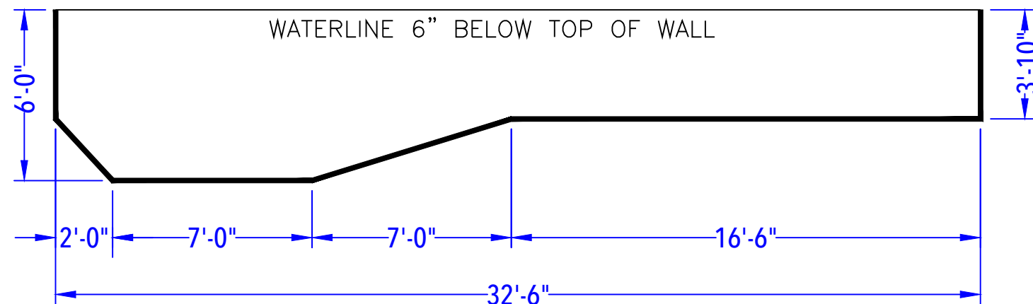
DEPTH DETAIL
