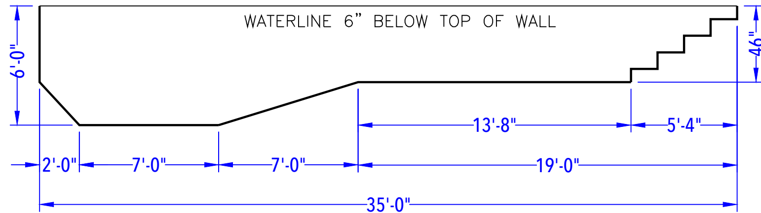
DEPTH DETAIL
