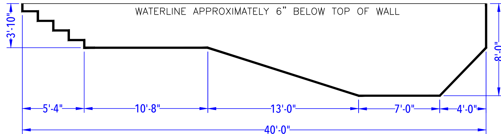
DEPTH DETAIL
