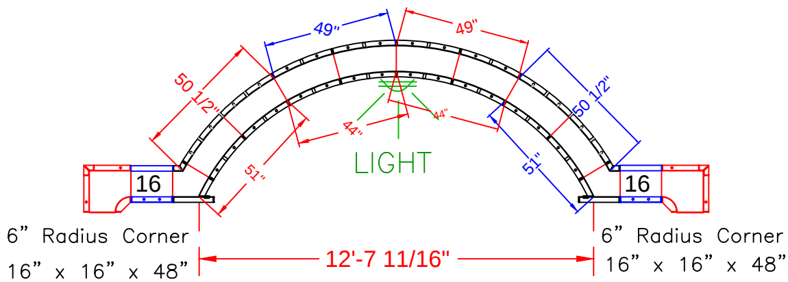
18' ROMAN END ASSEMBLY SHOWN x 48 SCALE: 1' = 1/4"
