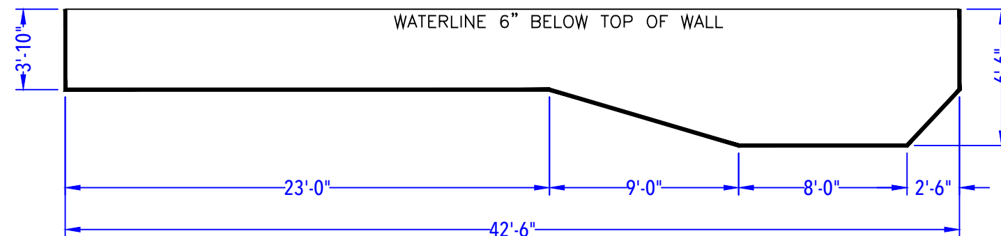
DEPTH DETAIL
