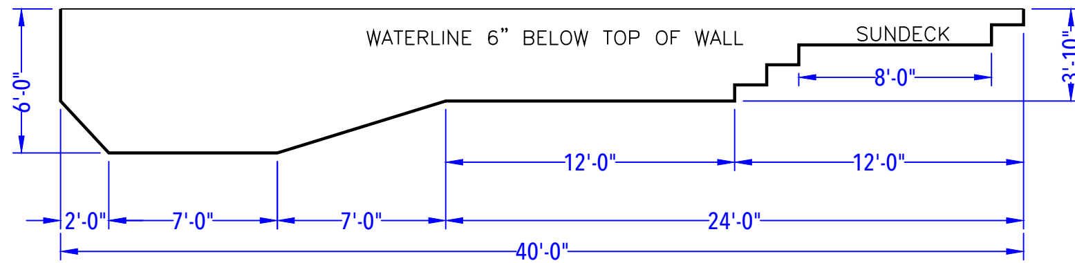
DEPTH DETAIL
