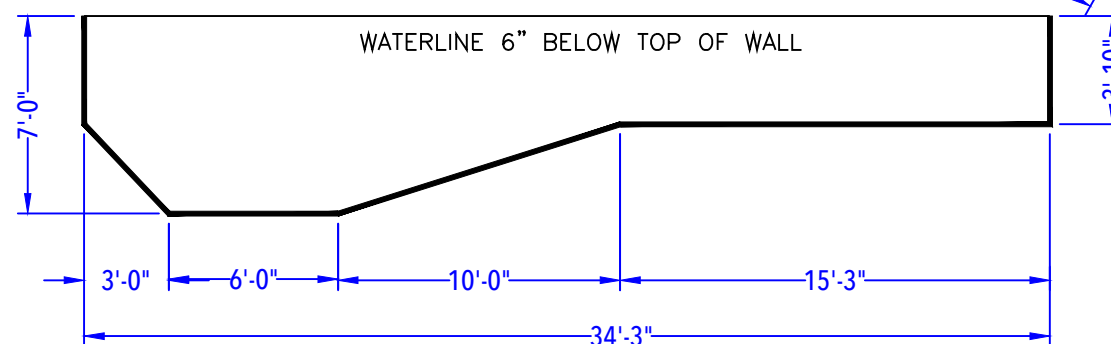
DEPTH DETAIL
