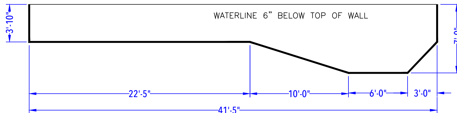
DEPTH DETAIL
