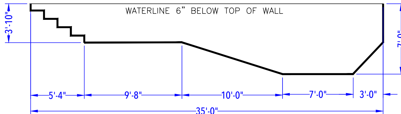
DEPTH DETAIL
