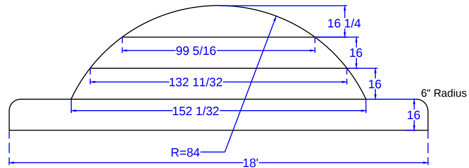
18' ROMAN END STEP ASSEMBLY SHOWN x 48 SCALE: 1' = 1/4"
