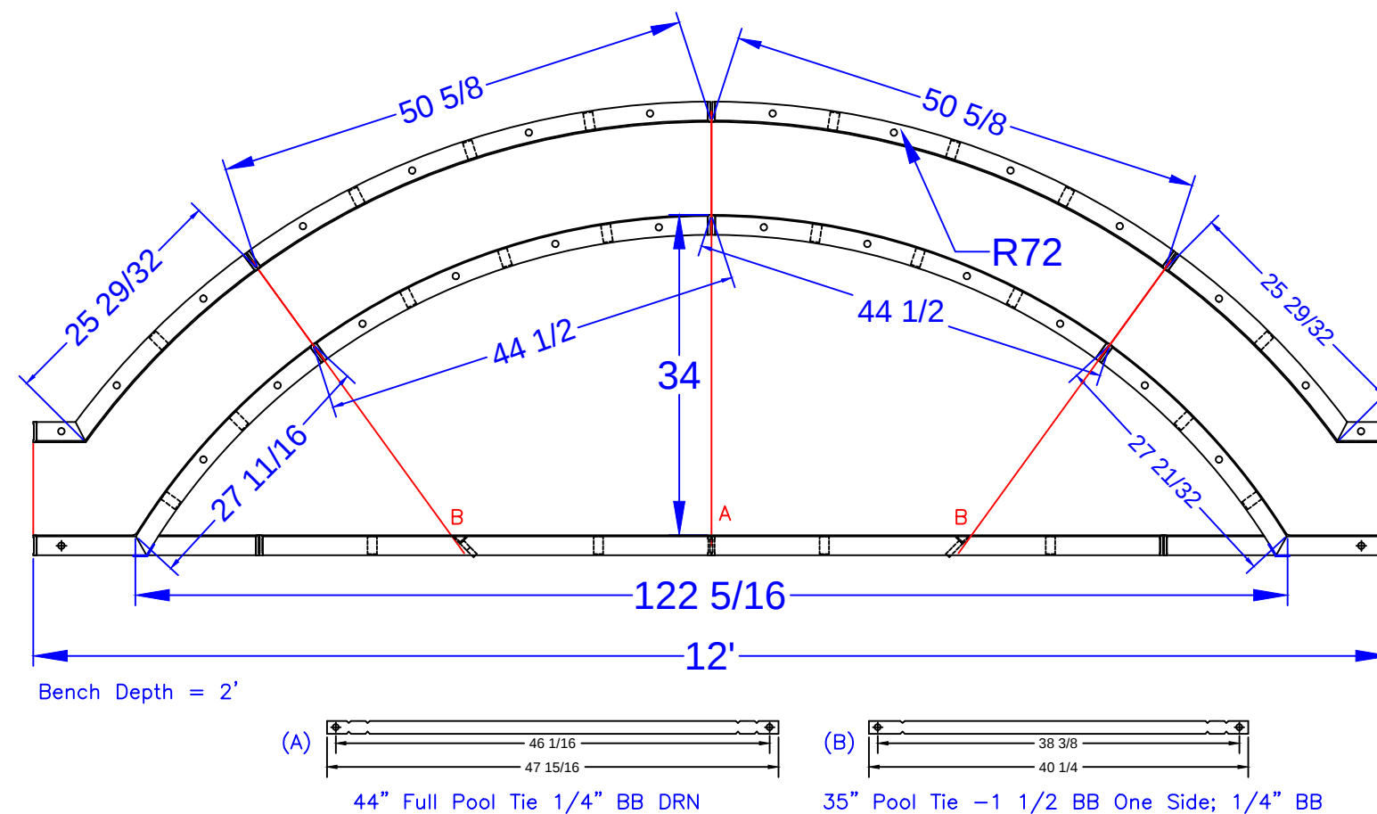
10'-2" ROMAN END LOVE SEAT (6' RADIUS) SCALE: 1' = 1/2"
