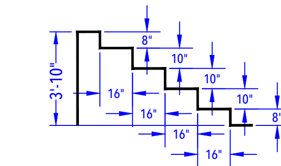
ENTRY STEP DETAIL (After Concrete & Liner) N.T.S.
