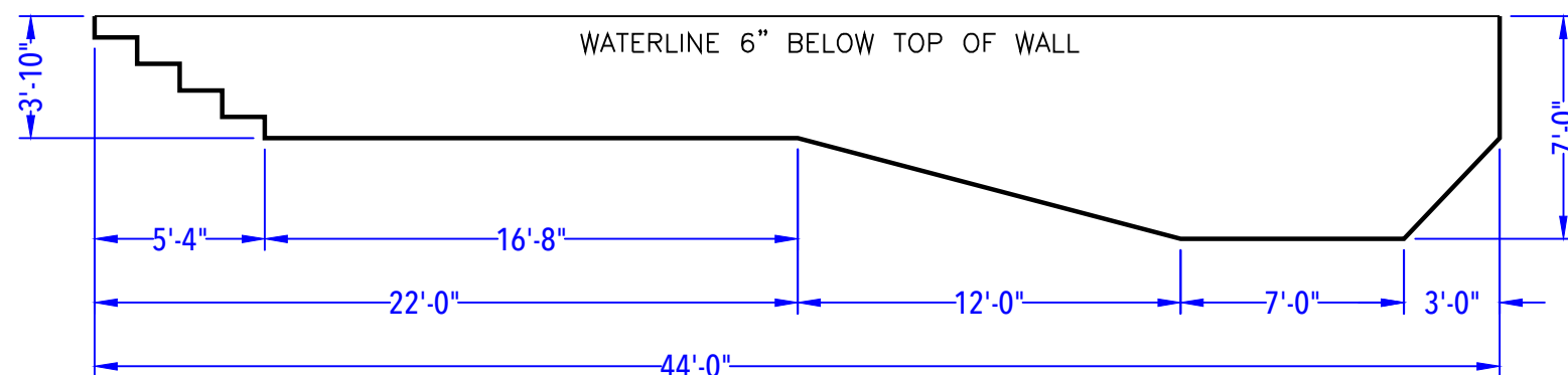
DEPTH DETAIL
