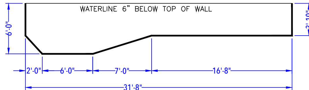
DEPTH DETAIL
