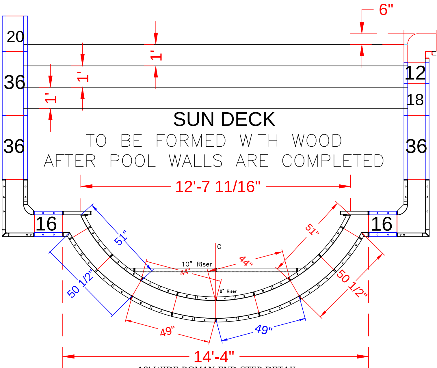
18' WIDE ROMAN END STEP DETAIL SCALE: 1' = 1 / 3 "
