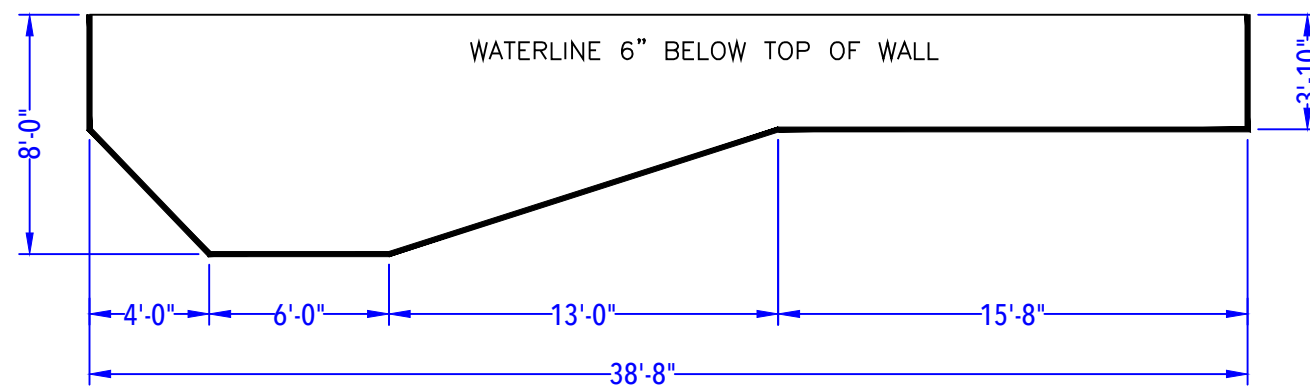
DEPTH DETAIL
