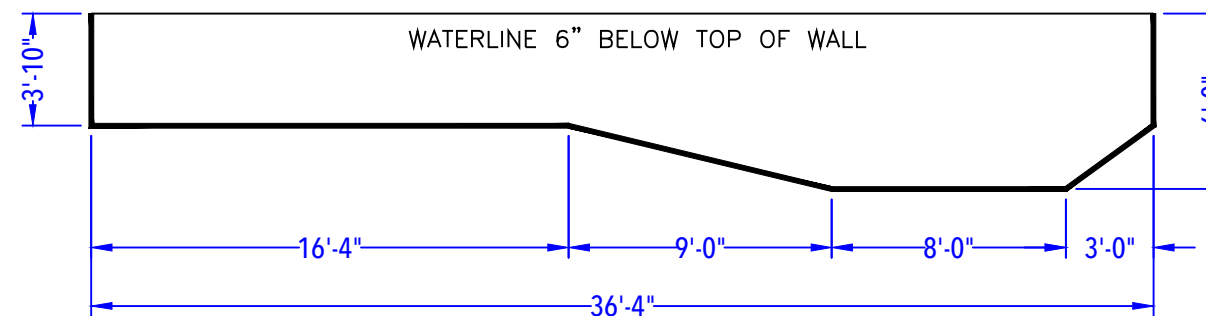
DEPTH DETAIL
