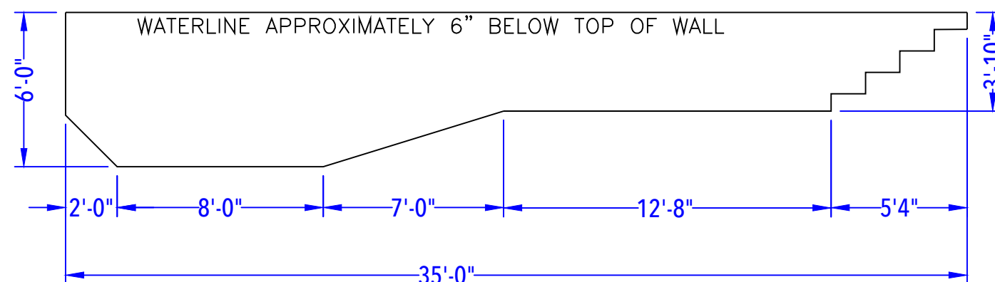
DEPTH DETAIL
