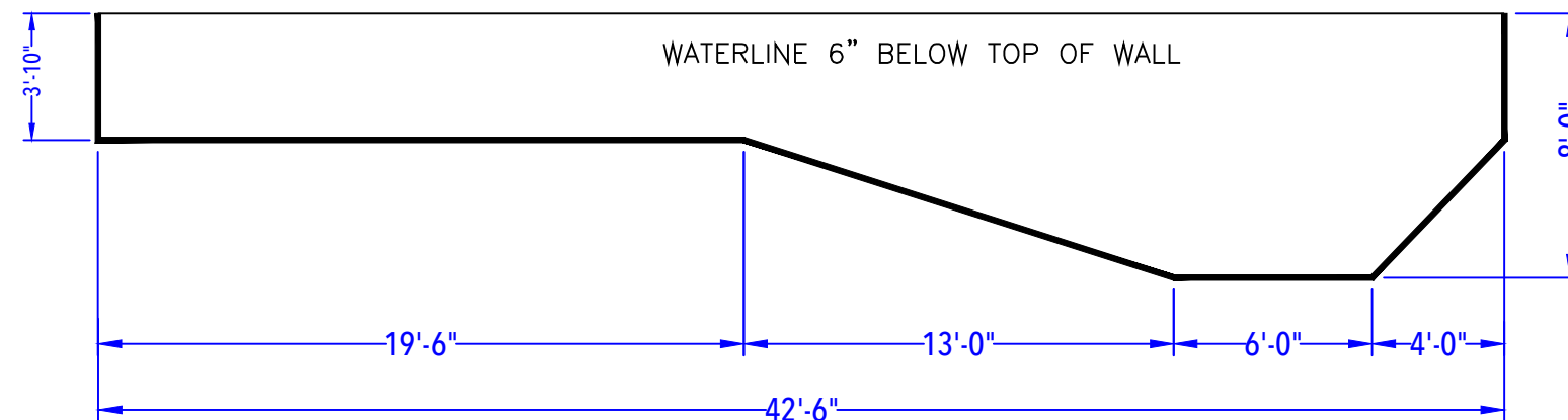
DEPTH DETAIL
