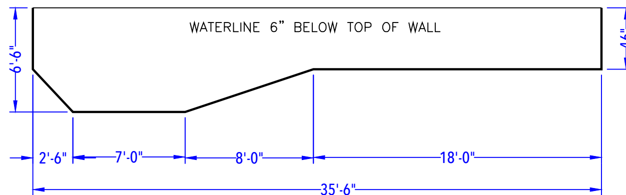
DEPTH DETAIL
